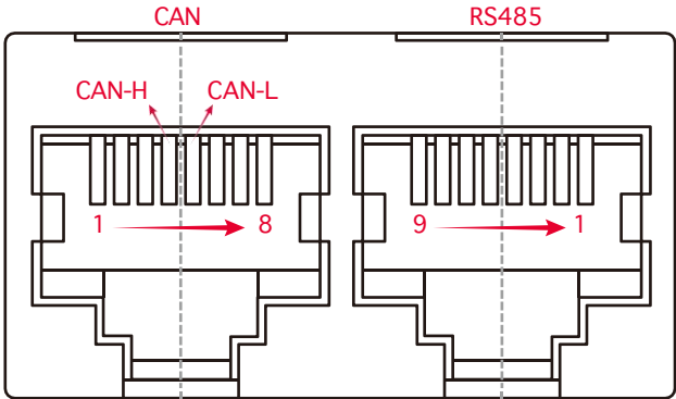
CAN and RS485 interfaces
